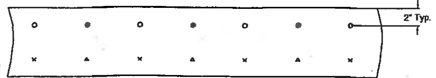
Stagger Pattern Plan and Elevation (Proposed Strip Floor) x ● ▲ ○ = Nail Row Designations
