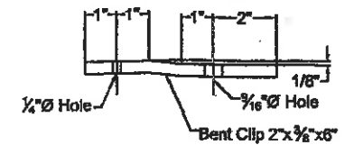
"Deck Securing" S-Clip Detail
