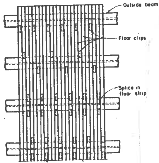
FLOOR CLIP LAYOUT
